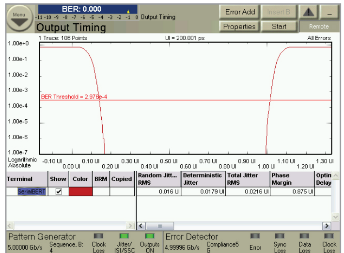
Figure 9. BERT scan including RJ/DJ separation, total jitter
