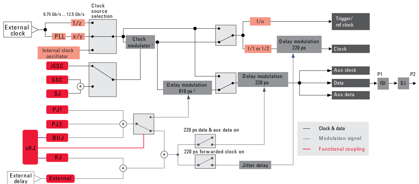
Figure 22. Overview of jitter injection capabilities
