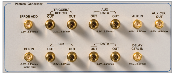
Figure 13. Generator connectors on front panel
