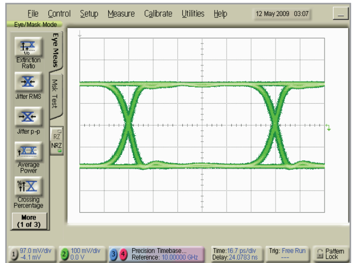
Figure 15. Clean output signal; 10 Gb/s, 400 mV amplitude
