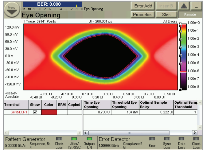
Figure 8. Eye contour with colors indicating BER level
