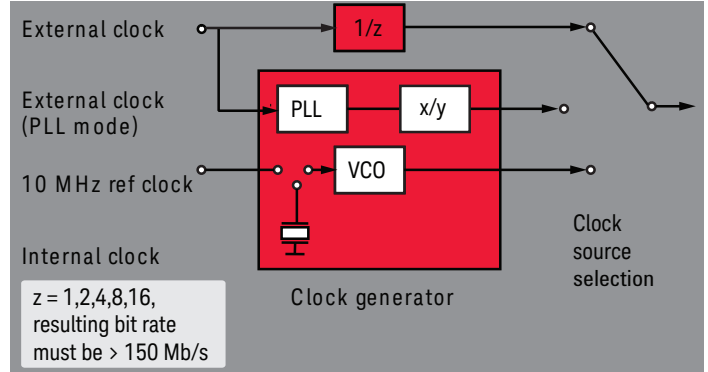
Figure 16. N4903B supports multiple clock modes
