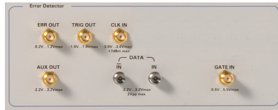
Figure 25. Front panel connectors for error detection
