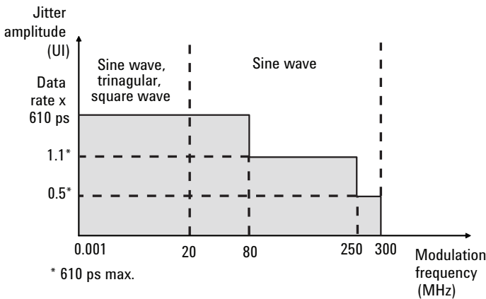
Figure 18. Periodic jitter maximum for data rates \leq 3.375 Gb/s using the 610 ps delay line
