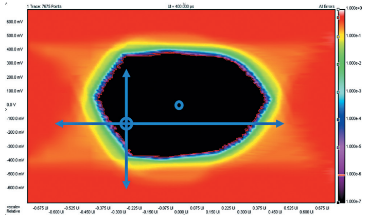
Figure 10. Bit recovery mode for analyzing non-deterministic traffic
