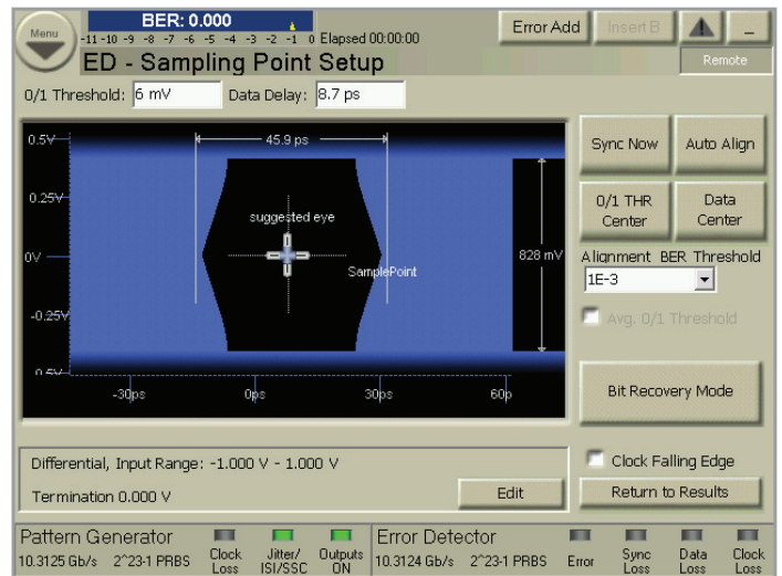
Figure 11. Auto alignment (center) simplifies correct sampling
