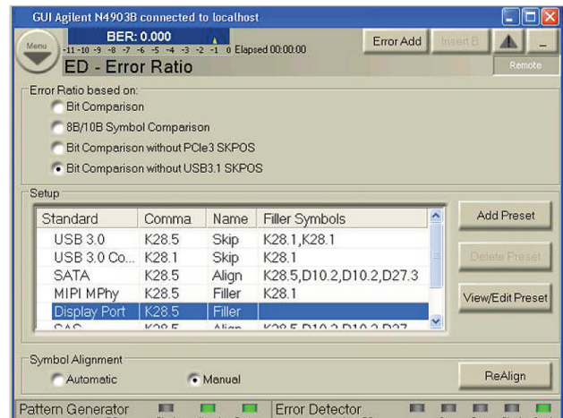
Figure 29. The analyzer options A02 and A03 enable error counting of devices such as PCIe, SATA, USB3.0 and USB3.1, that use retimed and coded loopback
