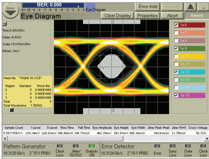
Figure 6. Quick eye diagram with BER contour and masking
